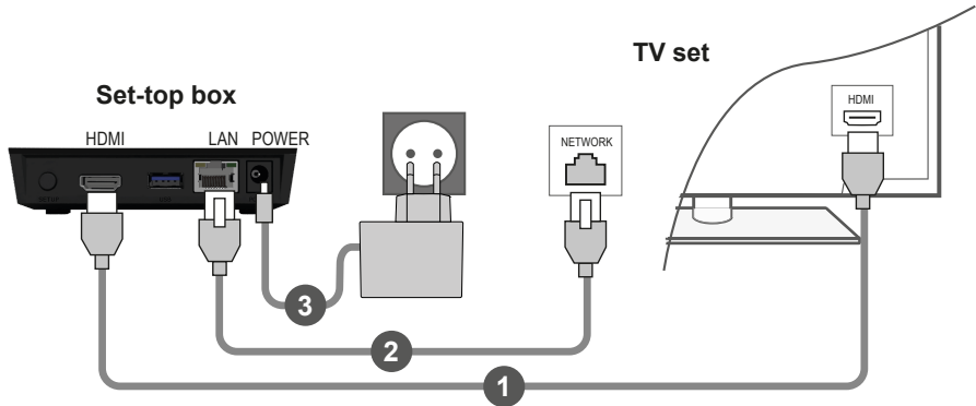
Figure 3: Cable connections
